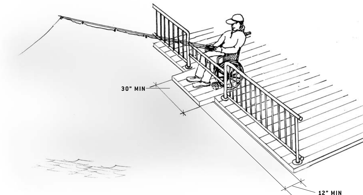
12-INCH DECK EXTENSION WITHOUT EDGE PROTECTION
